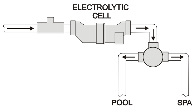
Inverted Installation
