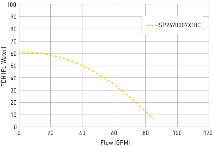
SUPER PUMP 700 FLOW VS. TOTAL HEAD
