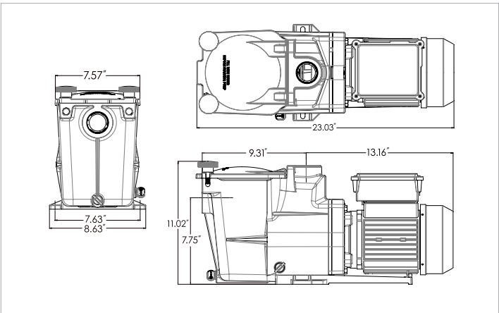
SUPER PUMP 700 DIMENSIONS (INCHES)
